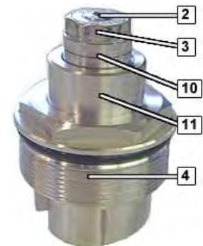
Fork cap with reversed preload
